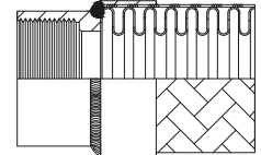
Threaded female end Manicotto filettato
