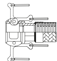
Camlock couplings Raccordi Camlock
