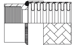
Manicotto filettato Threaded female end
